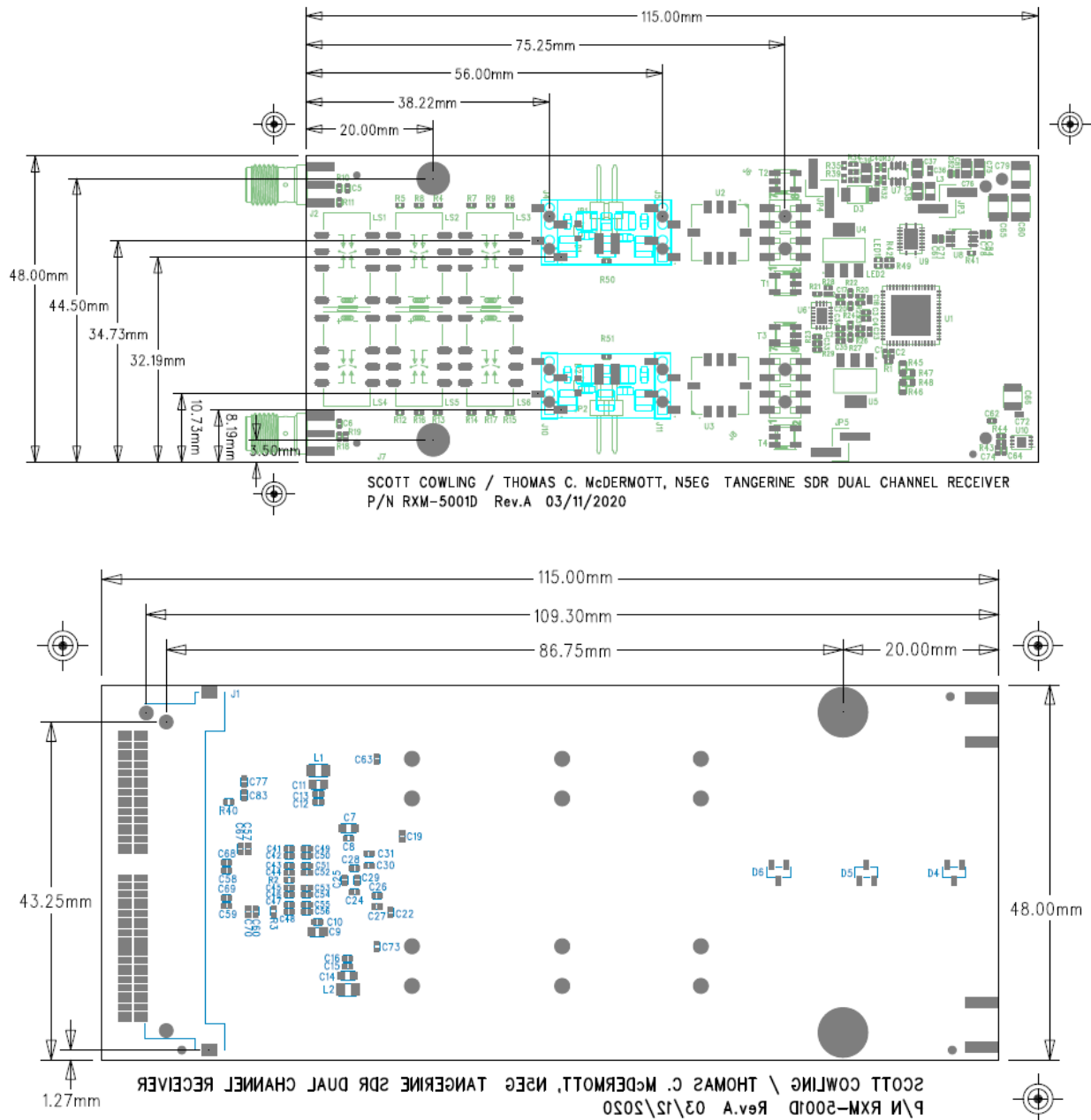
Figure 3 – Receiver Outline
